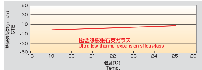
常温域の熱膨張係数 CTE at room temperature region
