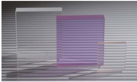
Nd:YAG ceramics
